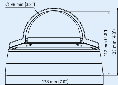
AXIS P3384-VE, AXIS P3346-VE, AXIS P3367-VE Weight: 1.7 kg (3.7 lb.) with weather shield
